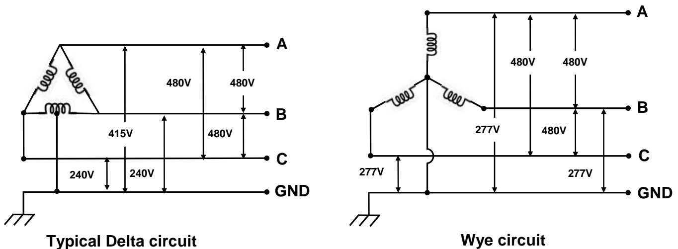
Figure 11: AC input wiring diagrams
