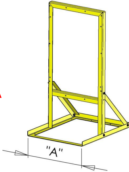
Figure 8: Shelf stand
