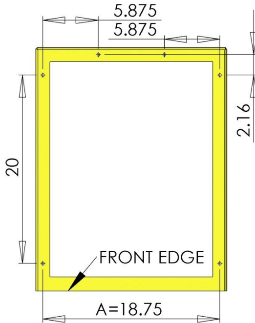
Figure 9: Shelf-stand mounting-bolt pattern
