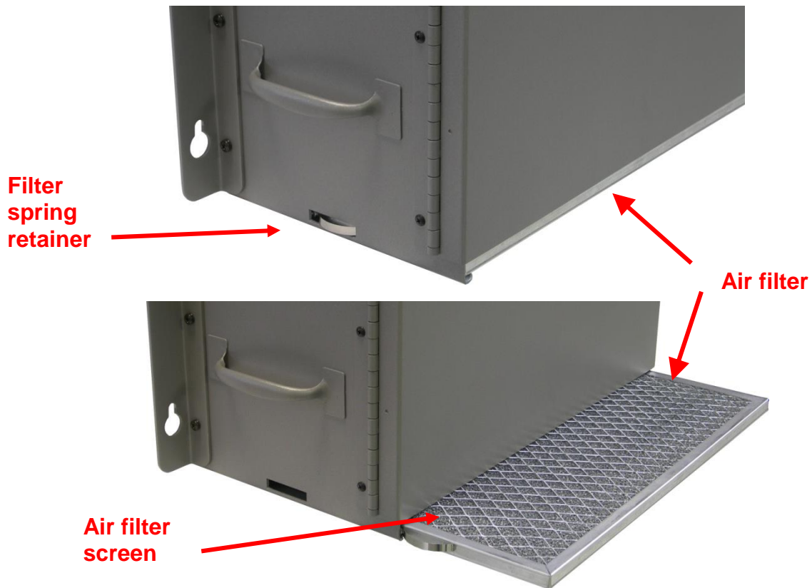
Figure 10: Installing/reinstalling the air filter
