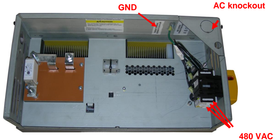
Figure 13: Charger electrical connection points
