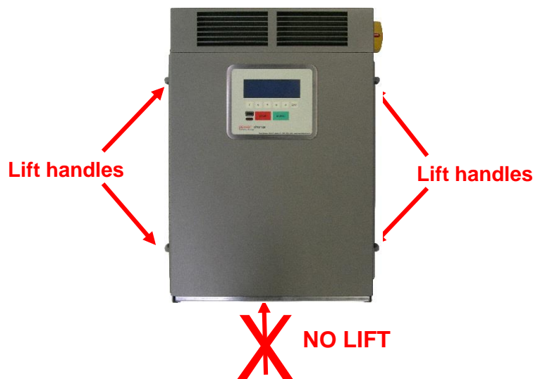
Figure 2: Charger lifting points
