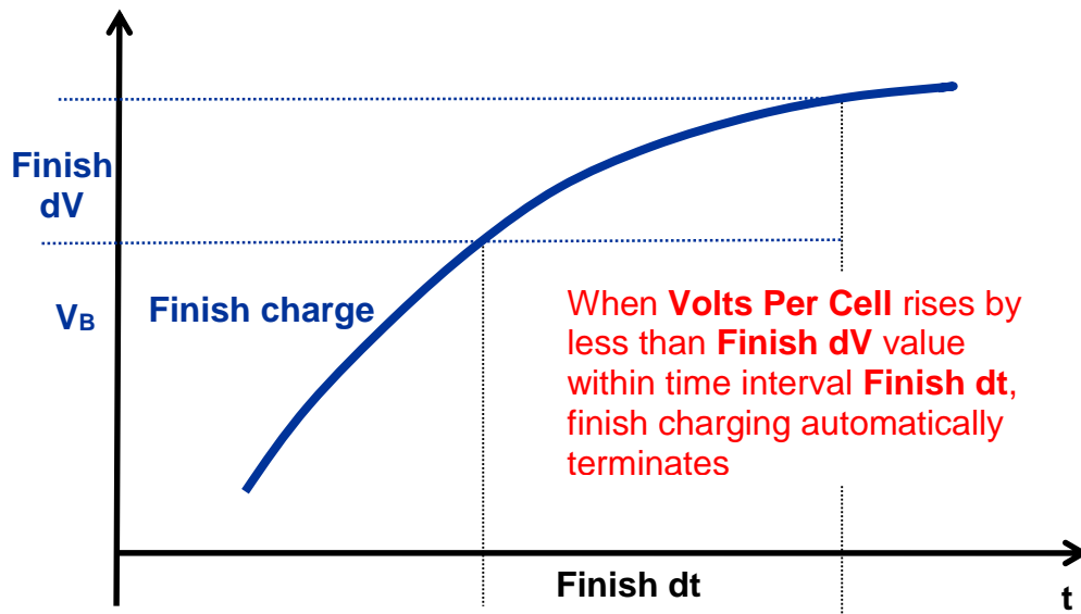
Figure 15: Finish charge termination criteria
